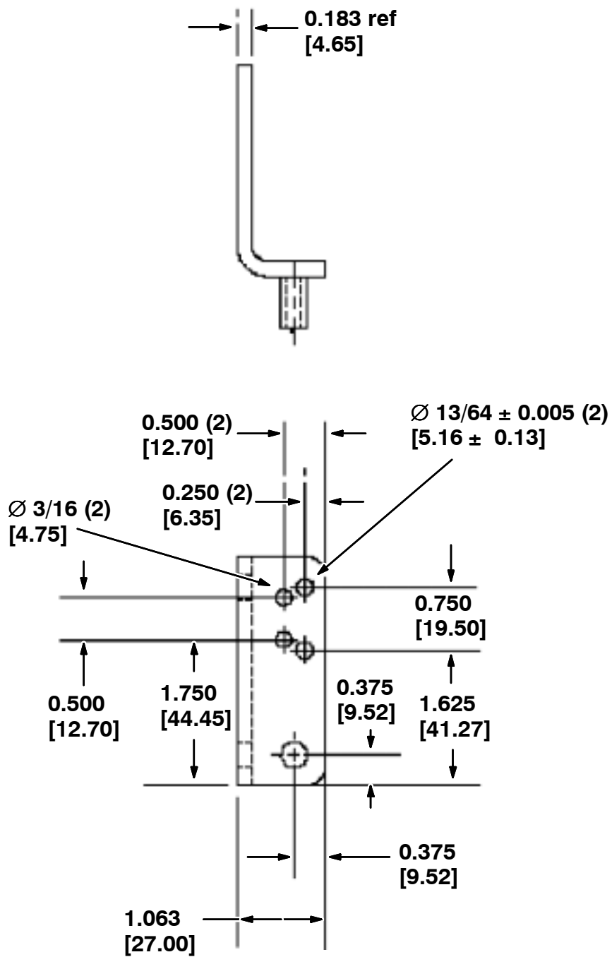
FIG. 2 - RIGHT HAND MOUNTING BRACKET REWORK
